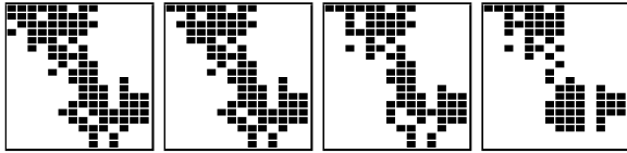
Figure 3. Context visualization (original, rank 8, 5, 3)
