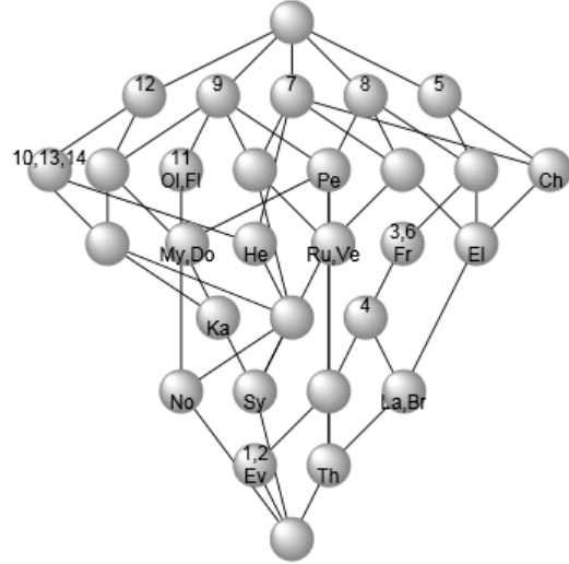
Figure 4. Galois lattice at rank 5
