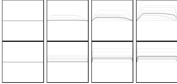
Figure 5. Lorenz curve comparing contexts (first row) and lattices (second row) - before and after reduction to ranks 8, 5, 3
