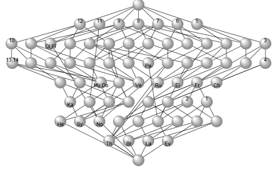
Figure 1. Galois lattice before reduction
